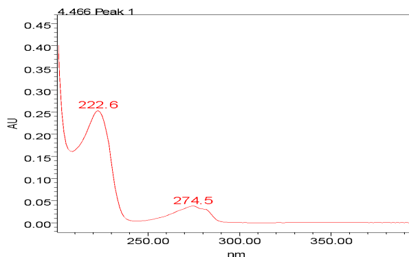
Fig. 1. PDA spectrum
