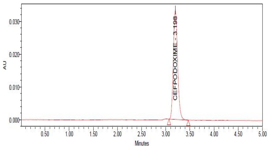
Fig. 12. Typical chromatogram of linearity 7.0 µg/ml
