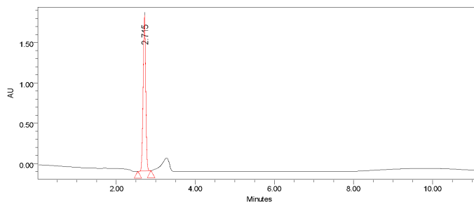
Fig. 5. Typical chromatogram trail 4
