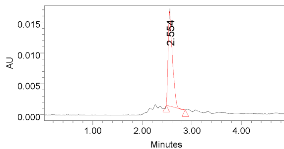
Fig. 3. Typical chromatogram trail 2
